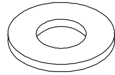
#132. Ø8.5 × 26 × 2.0T Flat Washer (2 pcs)
