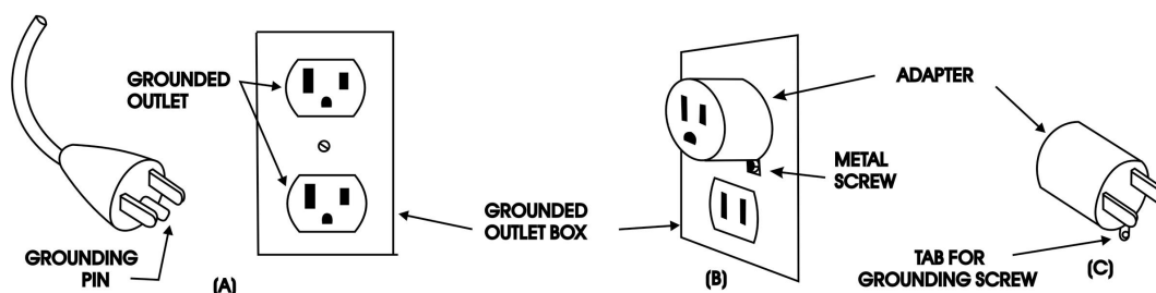
Grounding methods
